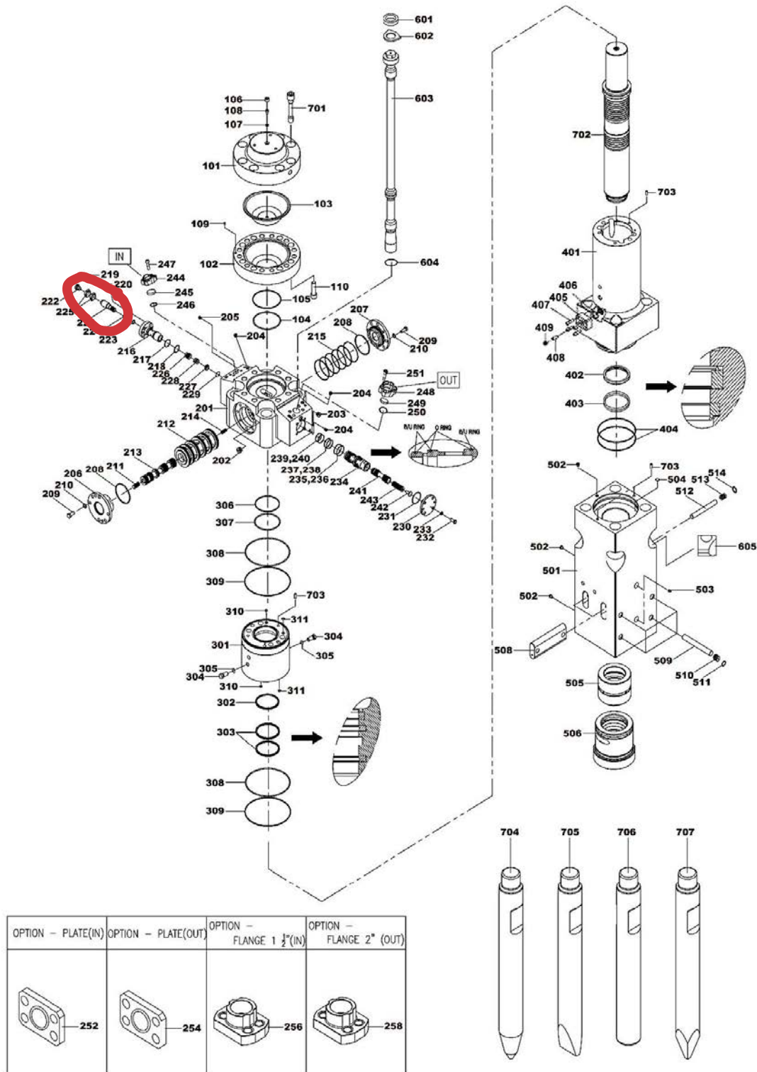
Figure 3.1 CH205 Breaker
