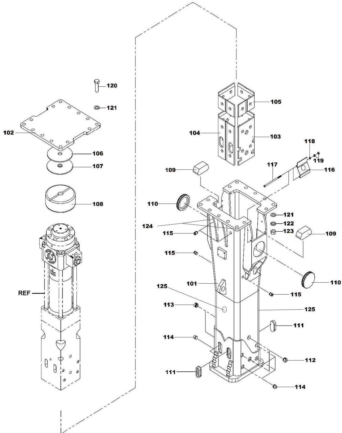
Figure 4.1 CH205 Housing
