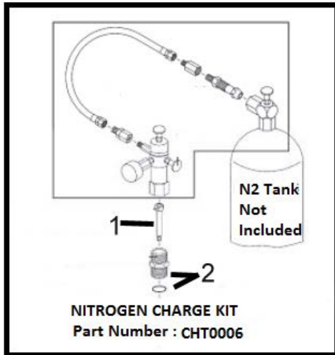
Figure 8.1 CH205 Nitrogen (N 2 ) Charge Kit
