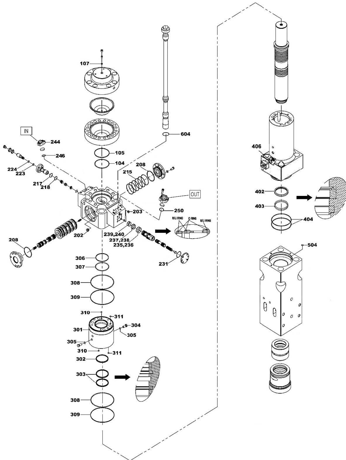
Figure 5.1 CH205 Seal Kit
